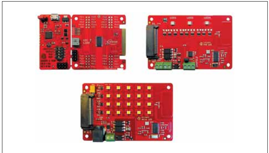
Рис. 3. Оценочная плата LED Lighting Application Kit с XMC1200
